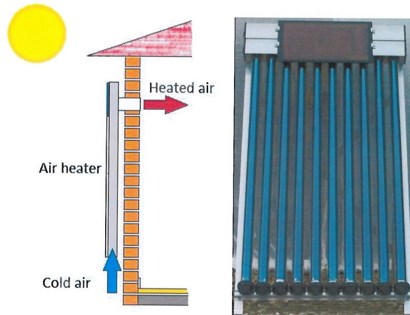
Figure 1: Drawing depicting the function of a solar air heater (left) the Ans Solvarme Vacpipe Open End 15/180/30 (right).
