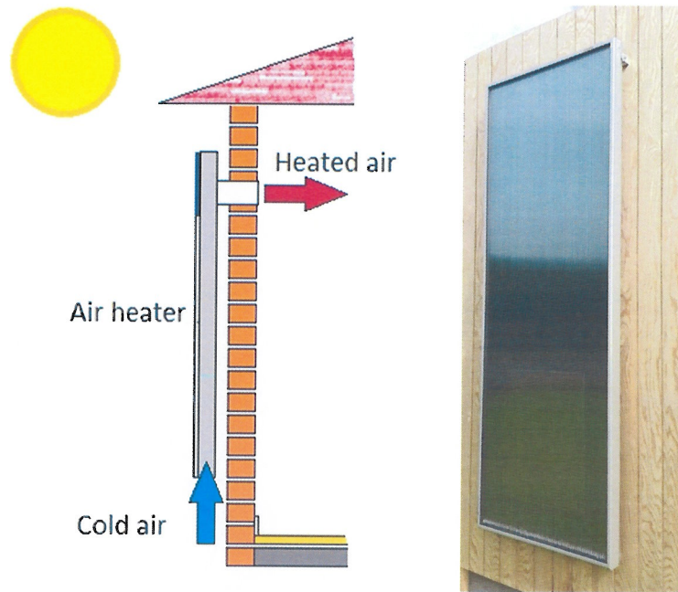
Figure 1: Drawing depicting the function of a solar air heater (left) and the SV14 solar air heater (right).
